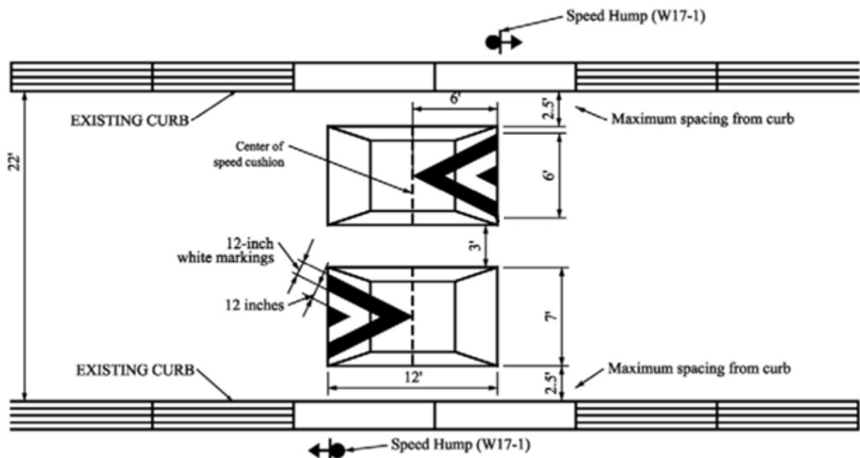
Speed Cushion Schematic with Median (DeIDOT)
