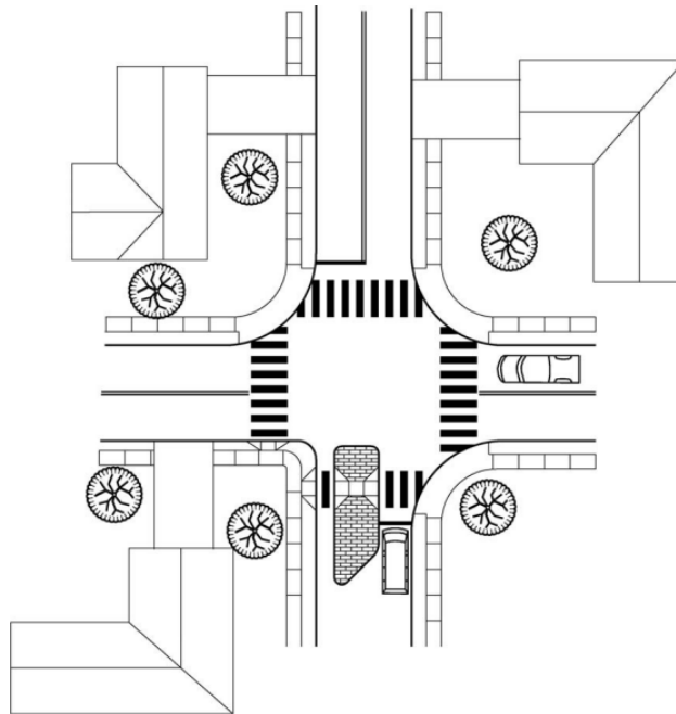
Partial Closure/Semi-Diverter (DeIDOT)
