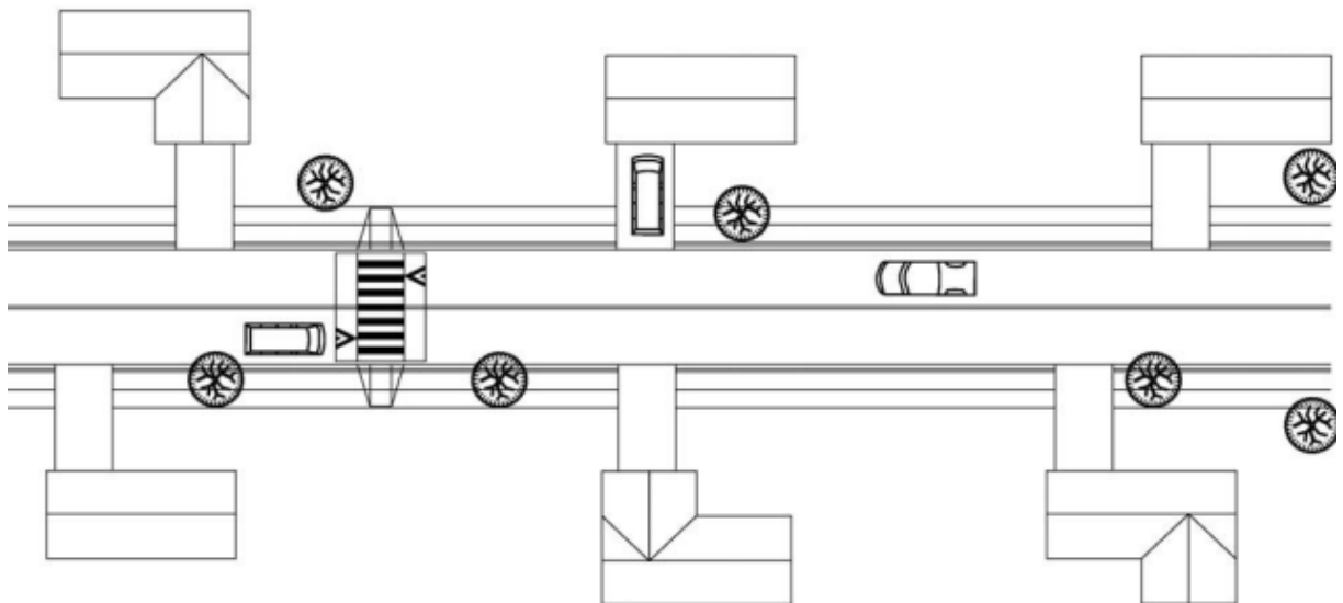
Speed Table / Raised Crosswalk (DeIDOT)
