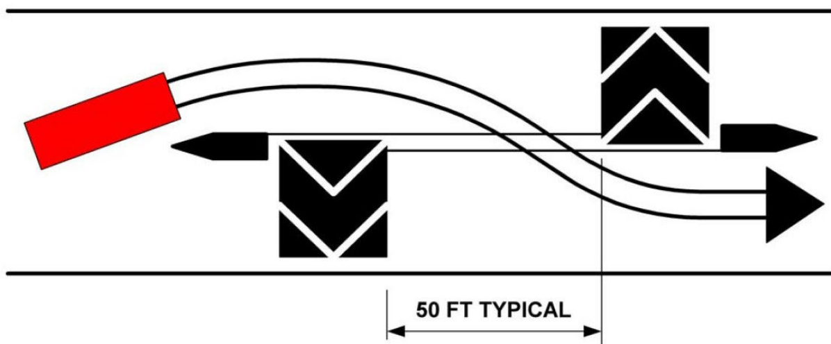
Offset Speed Table (NACTO, ITE)
