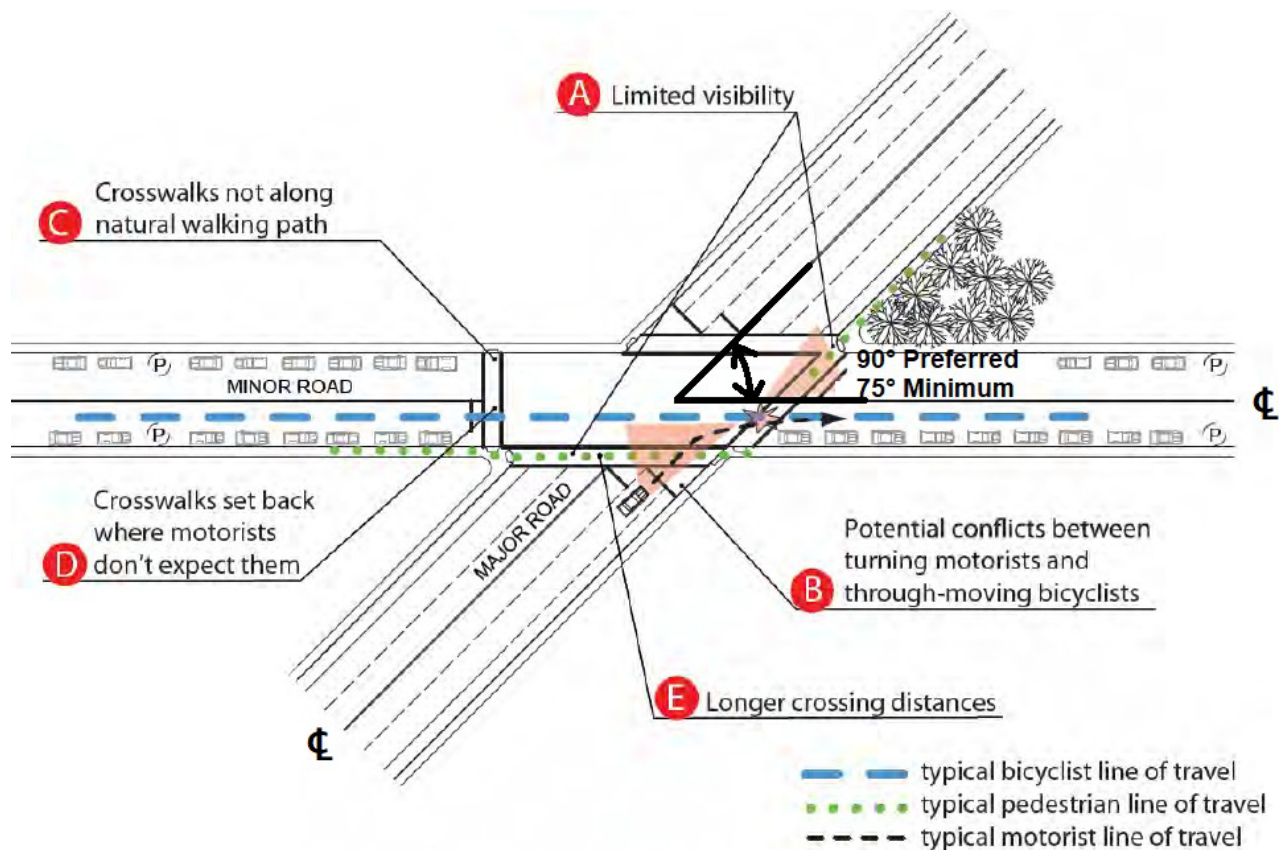
Minor Leg Skewed to the Right
