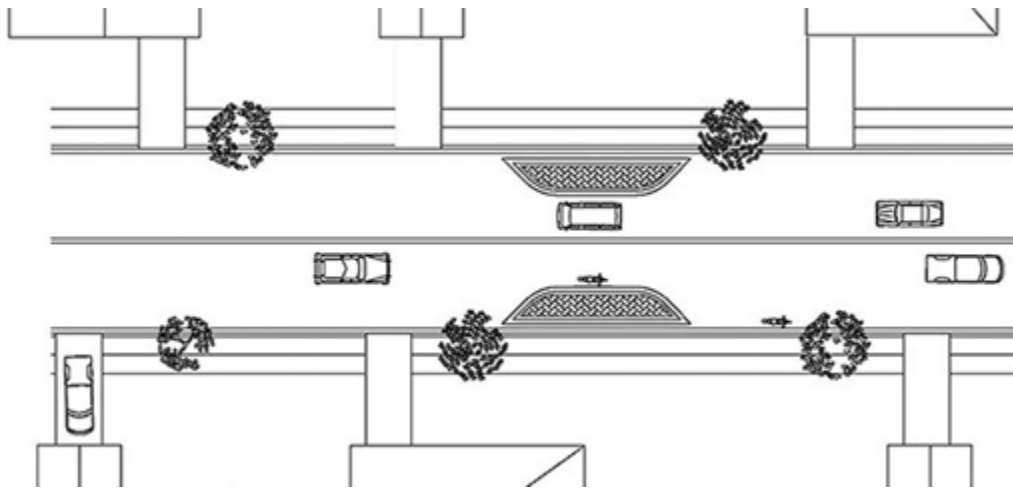
Choker Schematic (Source: Delaware Department of Transportation)
