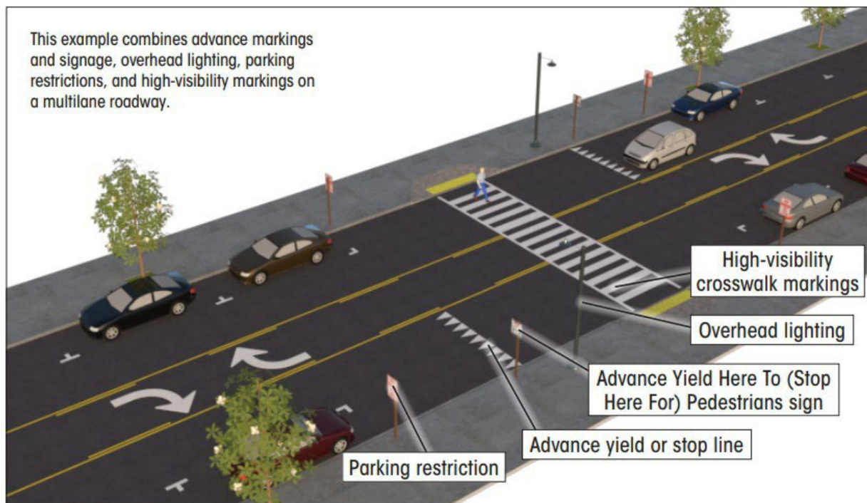
Crosswalk Enhancement Example (FHWA)
